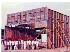
TRAIL ASSEMBLY OF 40 TON DUCT fabricated by M/s.VKN INDUSTRIES LENGTH:12700mm x WIDTH: 12500mm x HEIGHT:7036mm
